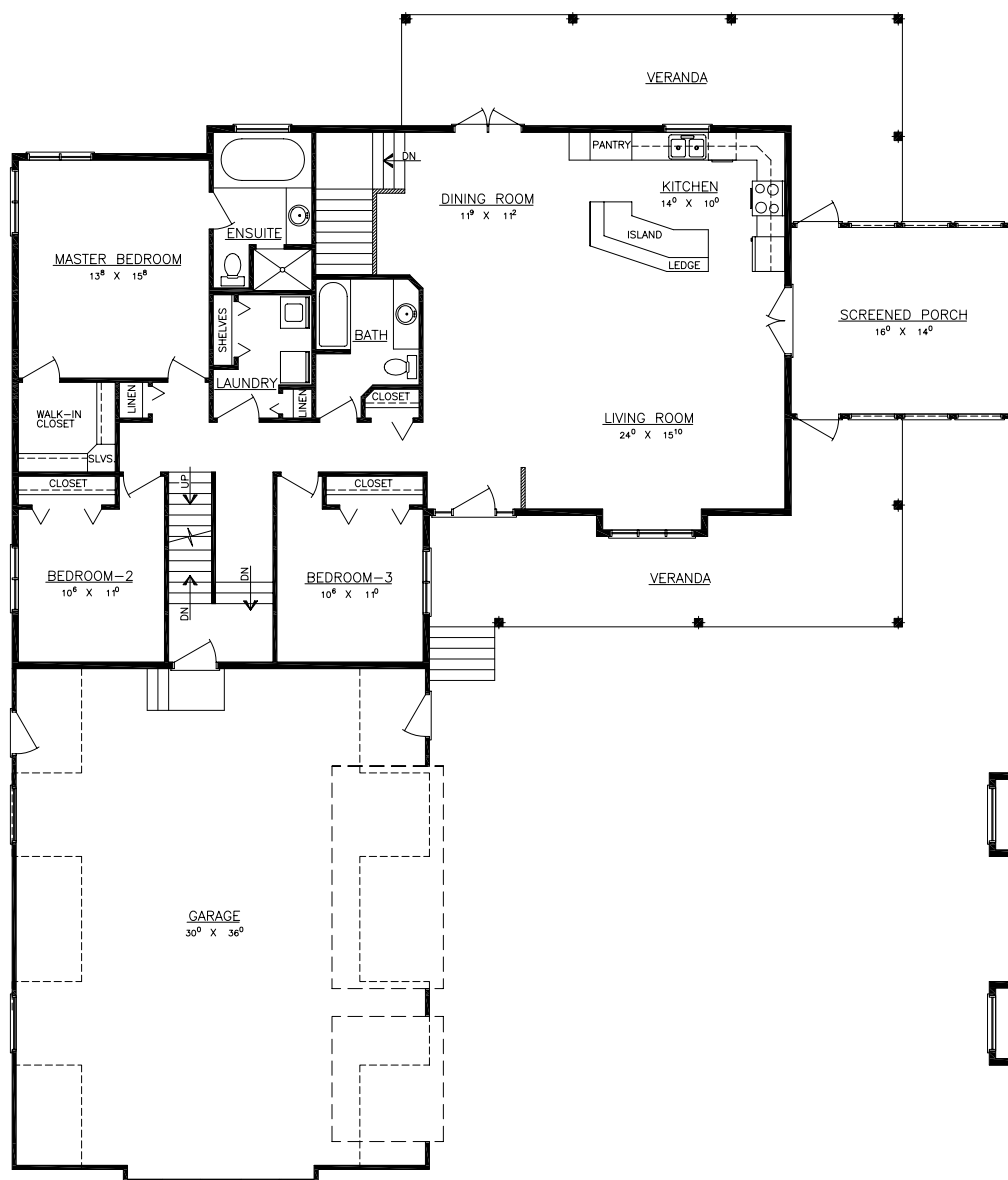
MAIN FLOOR
